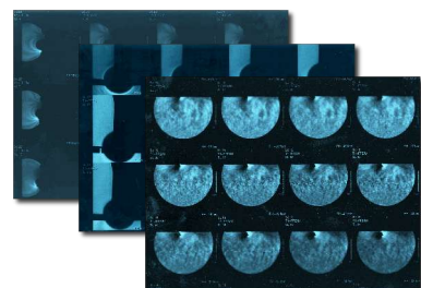
Different material samples with their MRI artefacts
