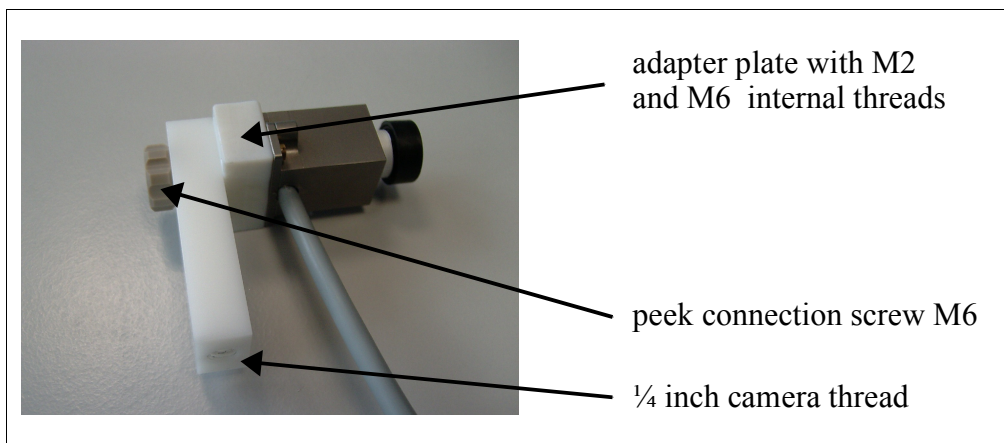
Figure 1: Application sample: adapter for tripod mounting
